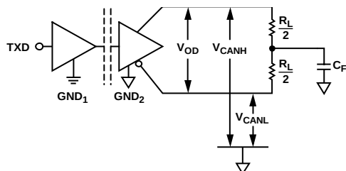
Figure 27. Driver Voltage Measurement
