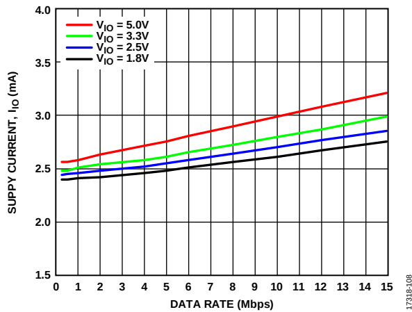
Figure 8. Supply Current, I_O vs. Data Rate
