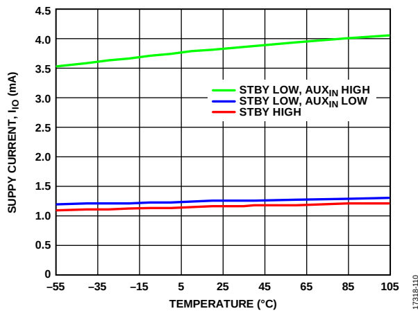
Figure 10. Supply Current, I_O vs. Temperature (Inputs Idle)
